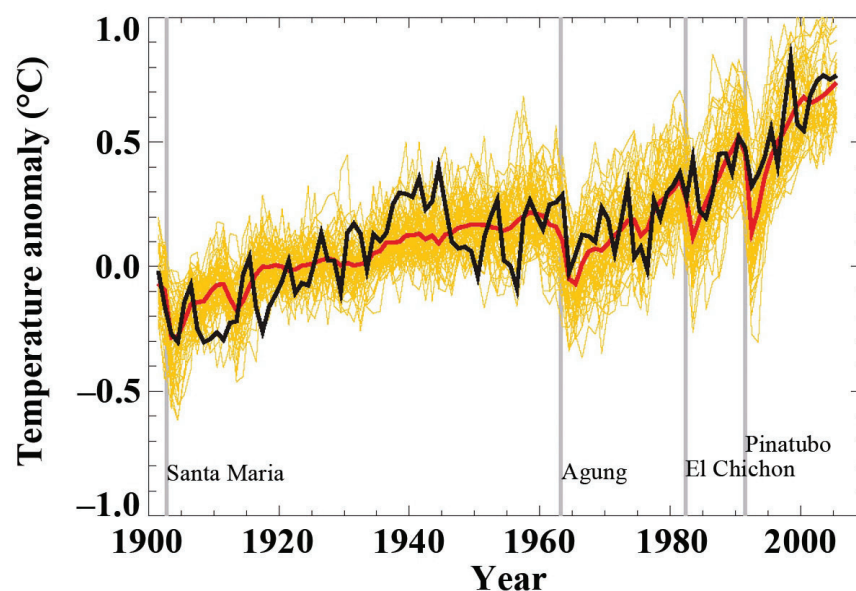
Figure 4 —Global near-surface mean temperature anomalies (relative to the 1901 to 1950 mean) observed for the 20 th century (black) and that simulated by fourteen different GCMs driven by natural and anthropogenic factors (yellow). The simulated mean is shown in red. Key volcanic eruptions are identified with vertical lines (gray) and labeled accordingly (source: AR4 WG1 Ch 8 p. 600).
